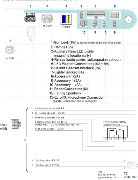
Plug connections inside radio box of the R 1200 RT-P:
